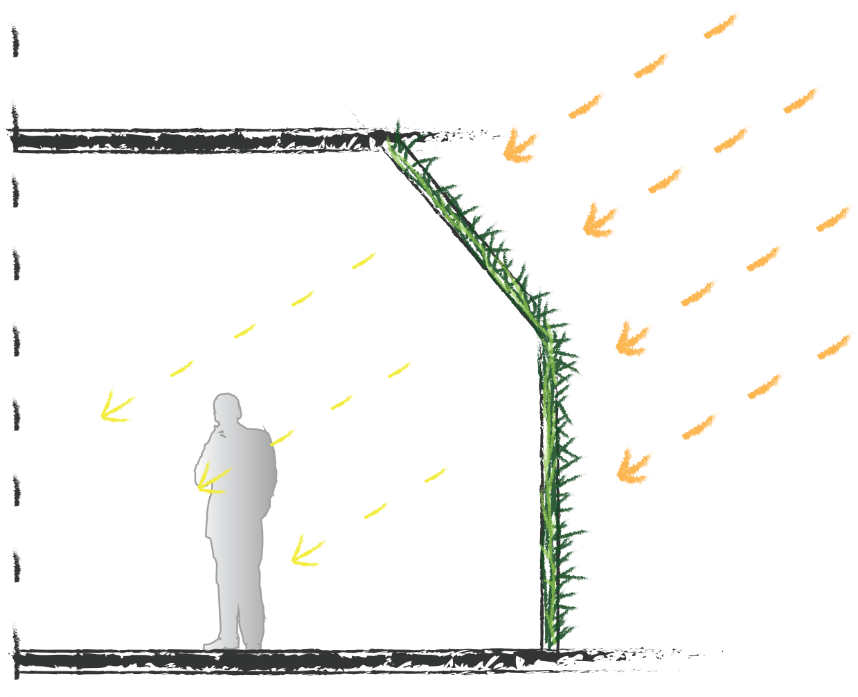
Filtering daylight and shading by use of moveable shields on the outer façade
